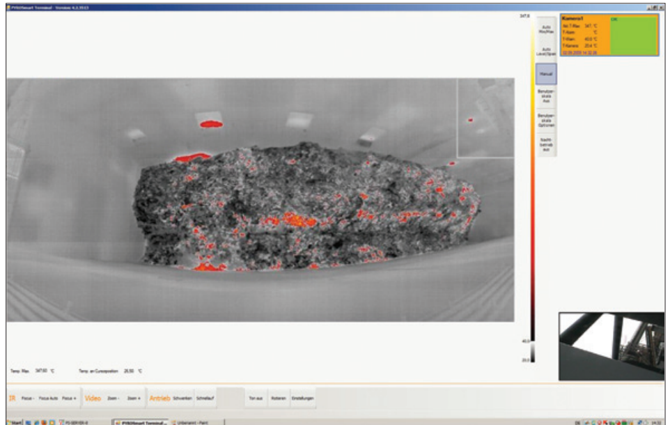
The PYROsmart system clearly shows the areas that are susceptible to spontaneous self combustion. The fire monitor will cool these areas down.
